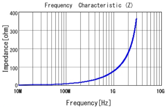
■ LQP02TN12NH02 |Z|
