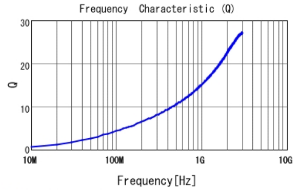
■ LQP02TN1N5B02 Q
