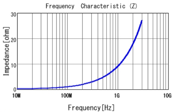
■ LQP02TN1N5B02 |Z|
