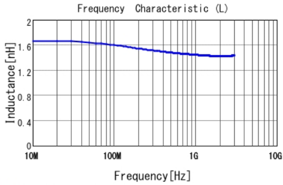
■ LQP02TN1N5B02 L
