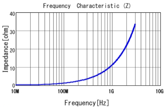
■ LQP02TN1N8B02 |Z|
