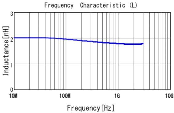
■ LQP02TN1N8B02 L
