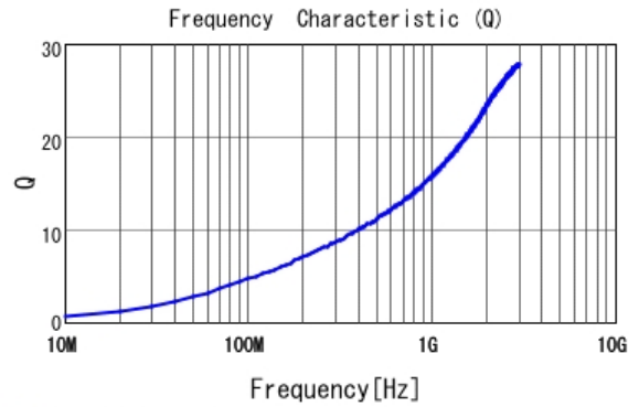
■ LQP02TN1N8B02 Q
