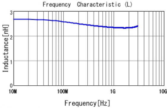
■ LQP02TN2N4B02 L
