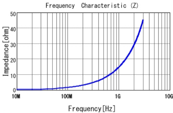
■ LQP02TN2N4B02 |Z|
