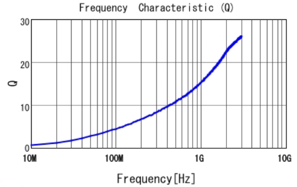
■ LQP02TN2N4B02 Q
