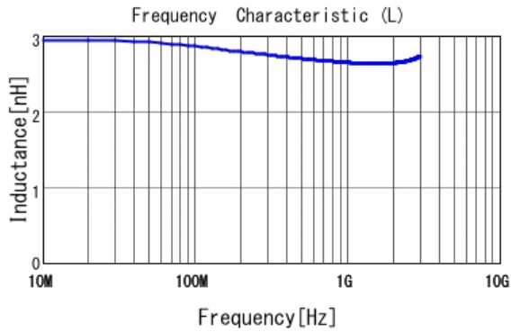
■ LQP02TN2N7B02 L
