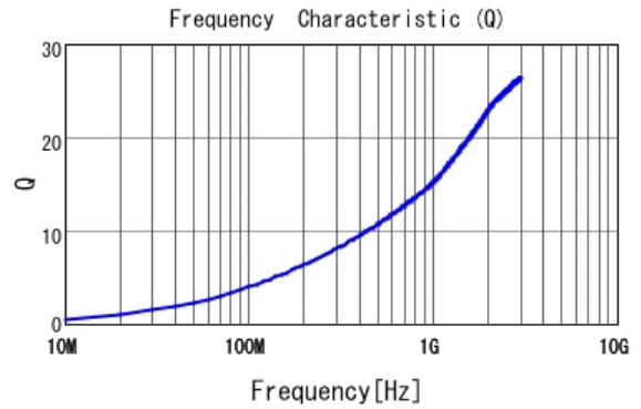
■ LQP02TN2N7B02 Q
