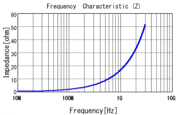
■ LQP02TN2N7B02 |Z|
