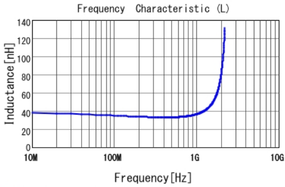
■ LQP02TN33NH02 L
