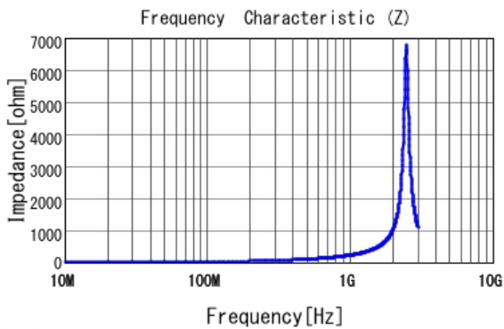
■ LQP02TN33NH02 |Z|
