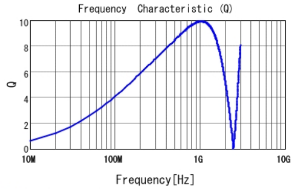
■ LQP02TN33NH02 Q
