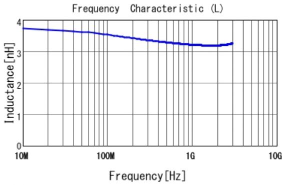
■ LQP02TN3N3B02 L
