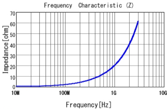
■ LQP02TN3N3B02 |Z|
