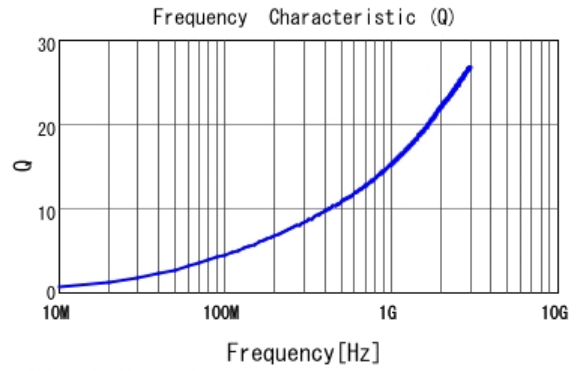
■ LQP02TN3N3B02 Q
