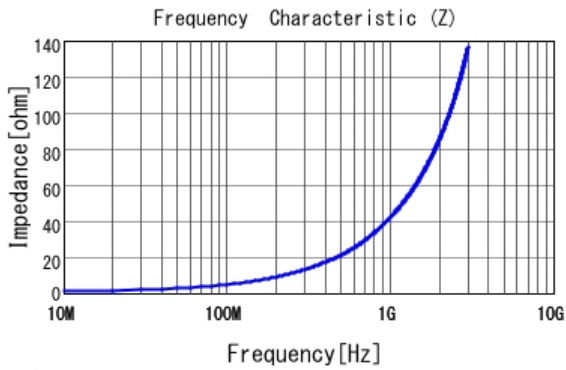
■ LQP02TN6N8H02 |Z|
