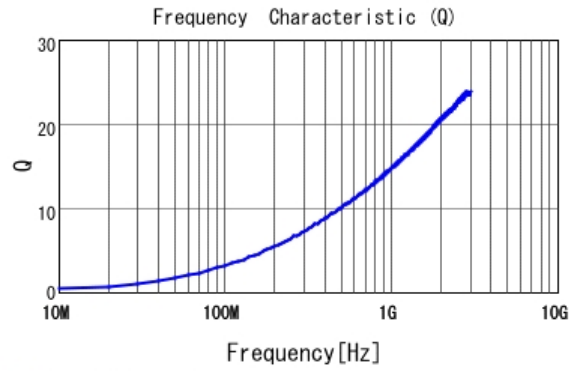
■ LQP02TN6N8H02 Q
