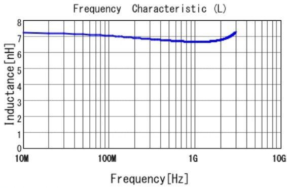
■ LQP02TN6N8H02 L
