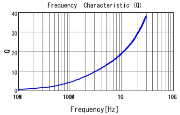
■ LQP02TQ3N4B02 Q
