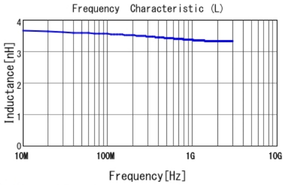
■ LQP02TQ3N4B02 L
