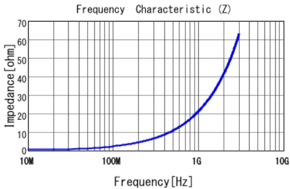
■ LQP02TQ3N4B02 |Z|
