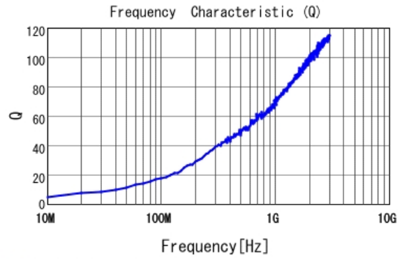
■ LQP03HQ1N0B02 Q
