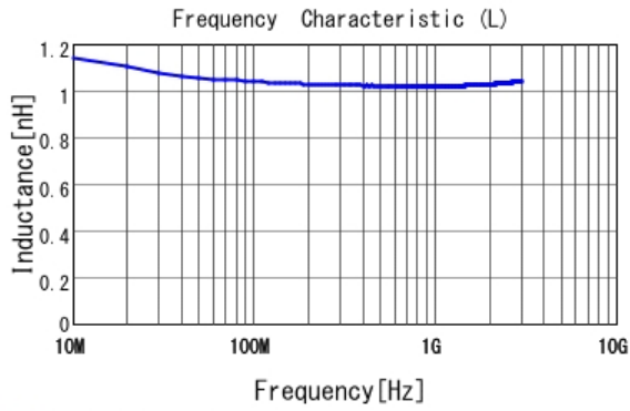
■ LQP03HQ1N0B02 L
