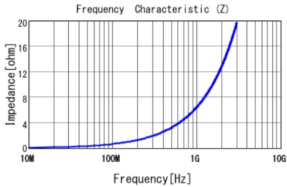
■ LQP03HQ1N0B02 |Z|
