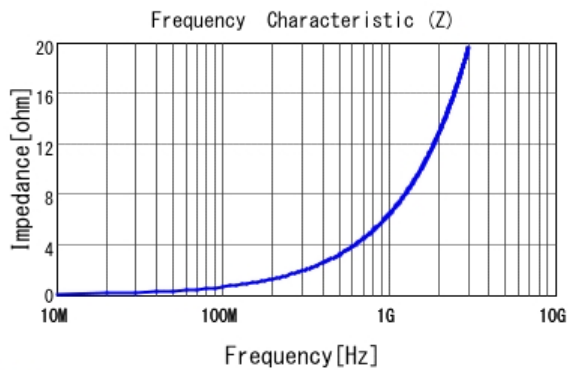
■ LQP03HQ1N0C02 |Z|
