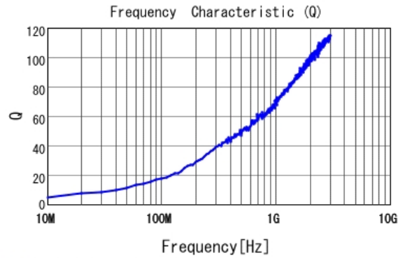
■ LQP03HQ1N0C02 Q
