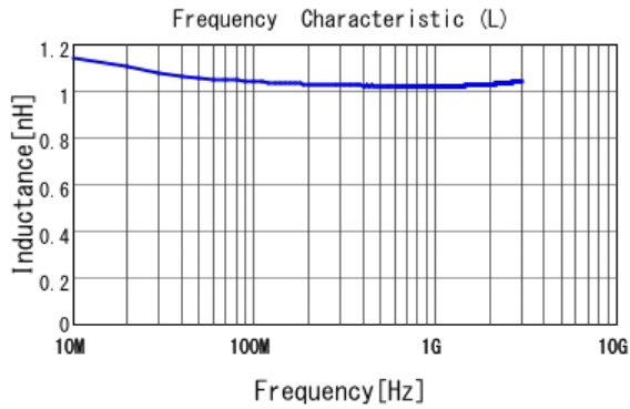
■ LQP03HQ1N0C02 L
