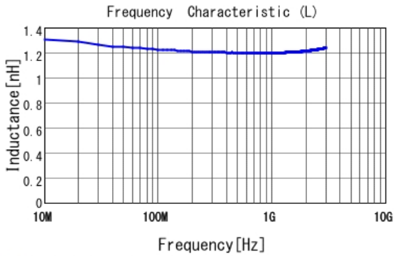
■ LQP03HQ1N2B02 L
