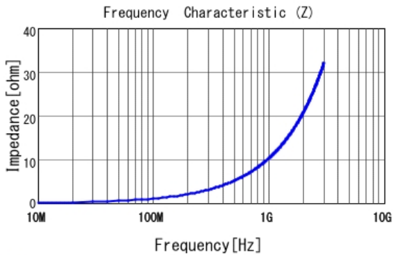
■ LQP03HQ1N6B02 |Z|
