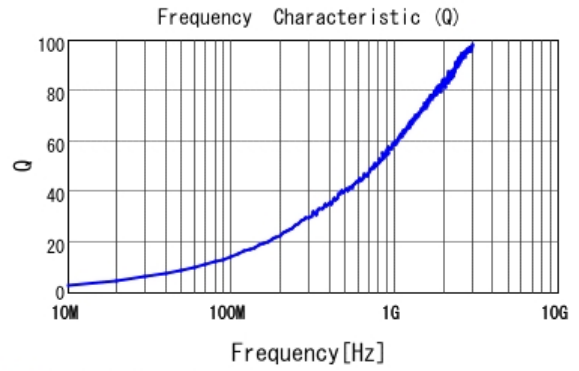
■ LQP03HQ1N6B02 Q
