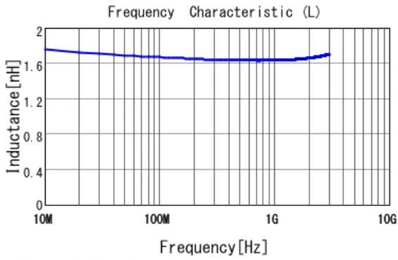
■ LQP03HQ1N6B02 L
