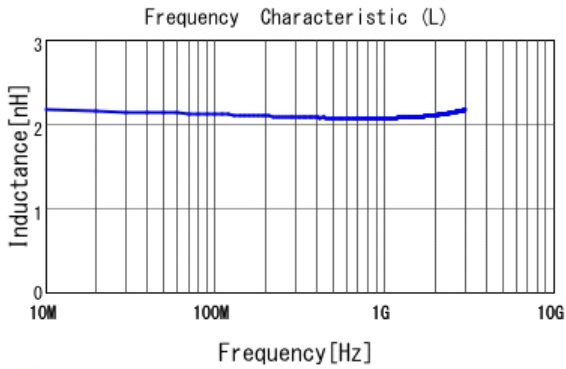
■ LQP03HQ2N0C02 L
