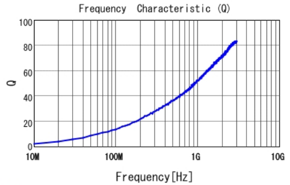
■ LQP03HQ2N0C02 Q
