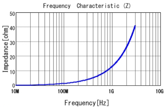
■ LQP03HQ2N0C02 |Z|
