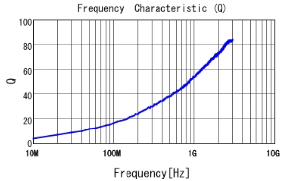
■ LQP03HQ2N2C02 Q
