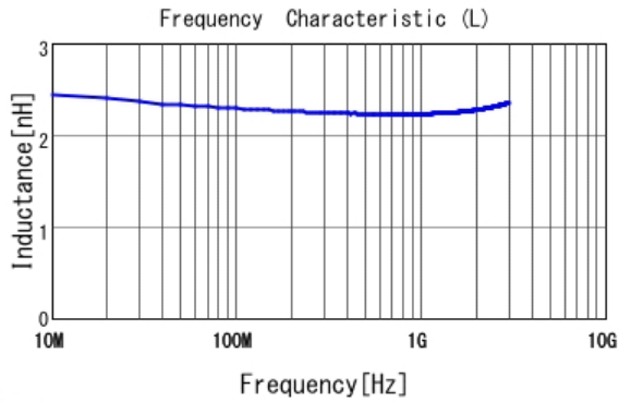
■ LQP03HQ2N2C02 L
