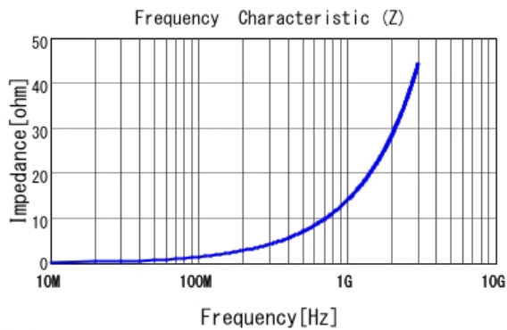
■ LQP03HQ2N2C02 |Z|
