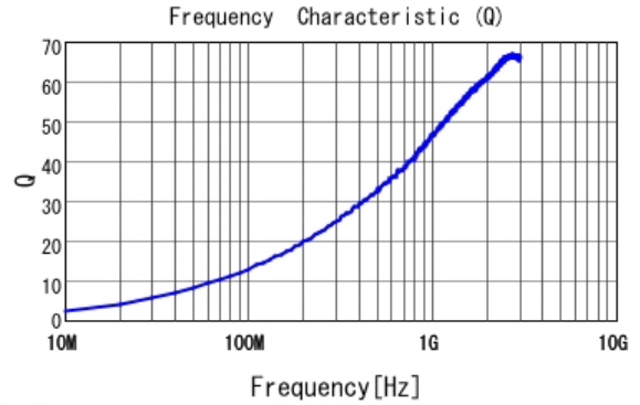
■ LQP03HQ3N6B02 Q
