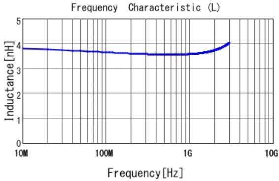
■ LQP03HQ3N6B02 L
