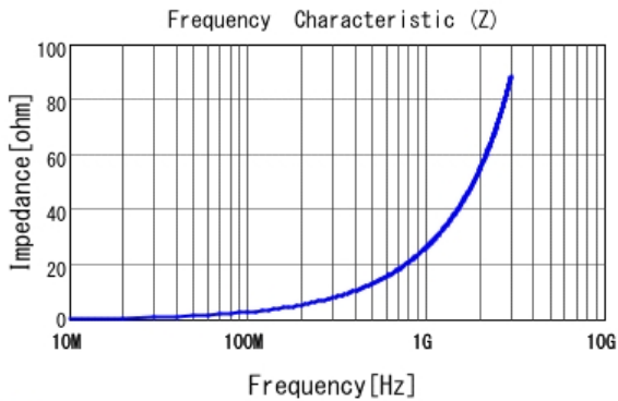
■ LQP03HQ4N1B02 |Z|
