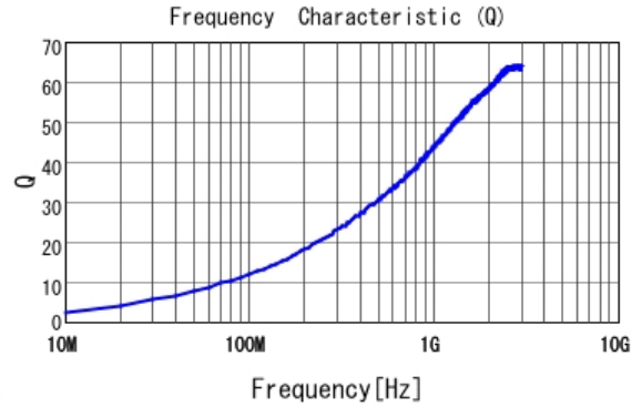
■ LQP03HQ4N1B02 Q
