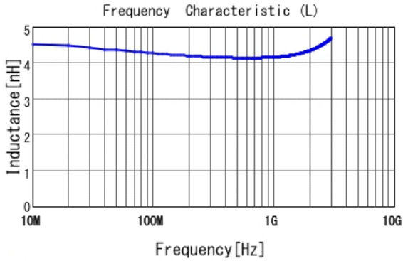
■ LQP03HQ4N1B02 L
