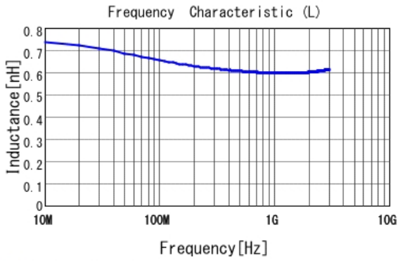
■ LQP03TG0N6B02 L
