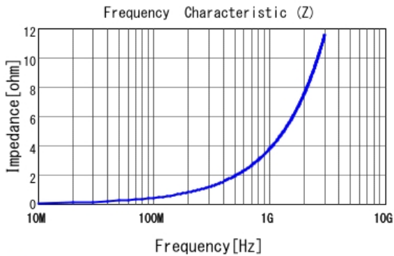
■ LQP03TG0N6B02 |Z|
