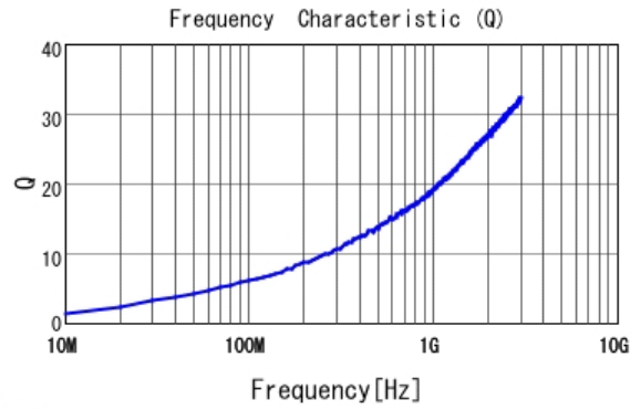
■ LQP03TG0N6B02 Q
