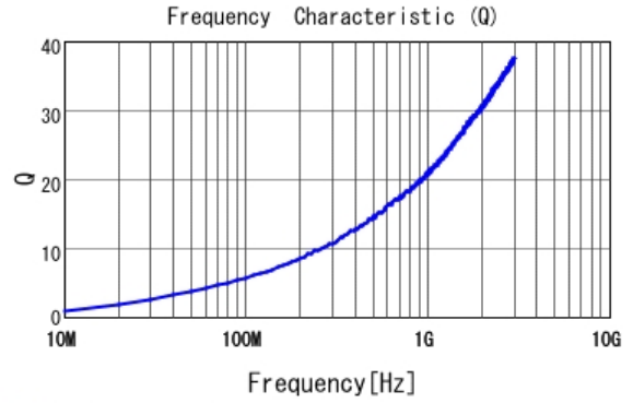
■ LQP03TG0N7B02 Q
