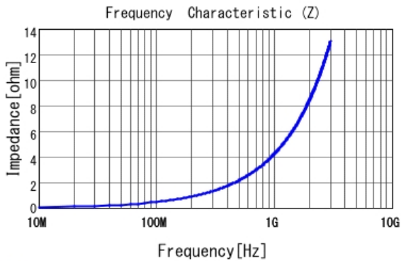
■ LQP03TG0N7B02 |Z|
