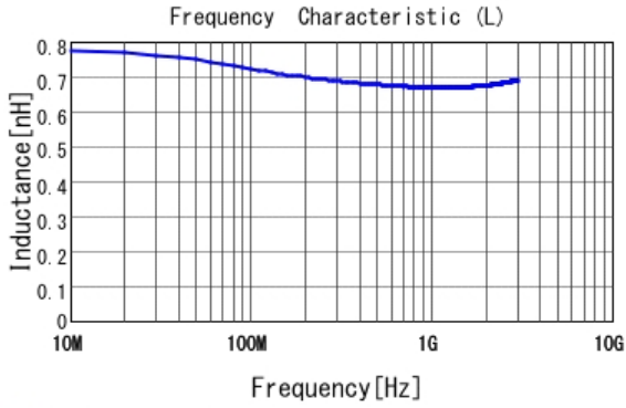
■ LQP03TG0N7B02 L
