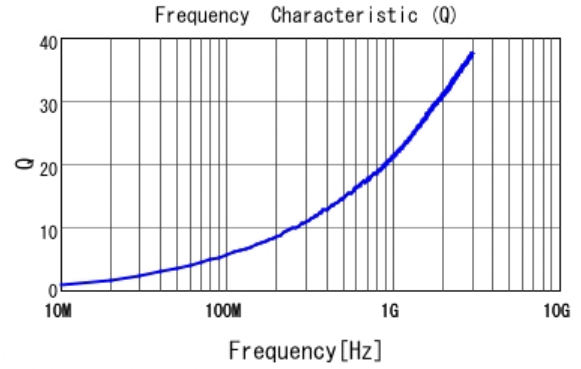
■ LQP03TG0N9B02 Q
