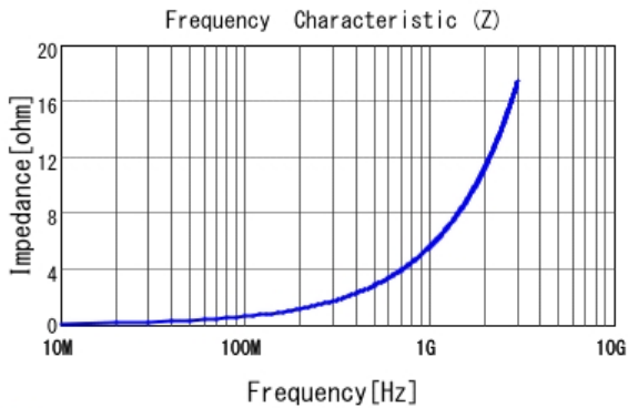
■ LQP03TG0N9B02 |Z|
