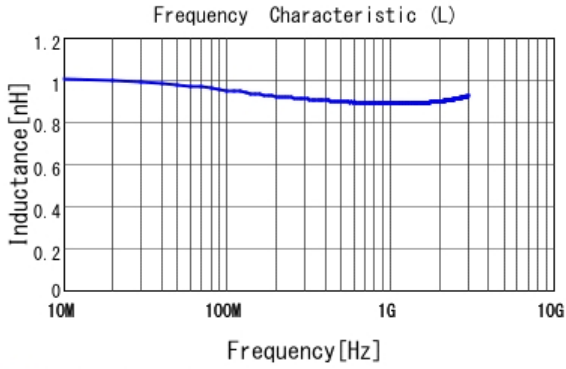
■ LQP03TG0N9B02 L
