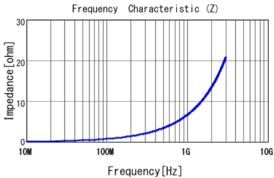
■ LQP03TG1N1B02 |Z|
