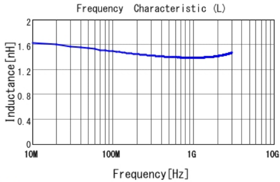
■ LQP03TG1N4B02 L
