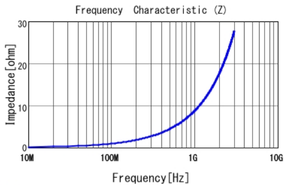
■ LQP03TG1N4B02 |Z|
