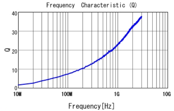
■ LQP03TG1N4B02 Q
