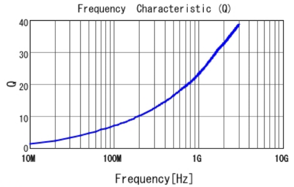
■ LQP03TG1N5B02 Q
