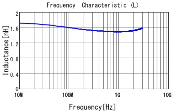
■ LQP03TG1N5B02 L
