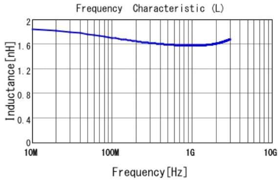
■ LQP03TG1N6B02 L
