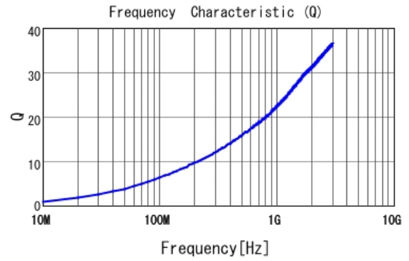
■ LQP03TG2N0B02 Q
