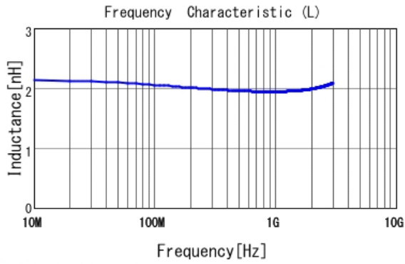
■ LQP03TG2N0B02 L
