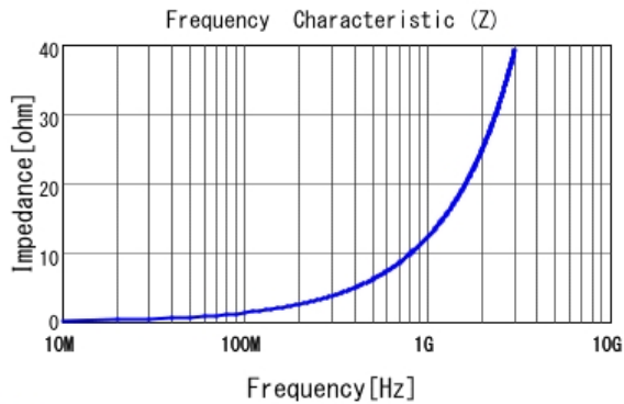
■ LQP03TG2N0B02 |Z|
