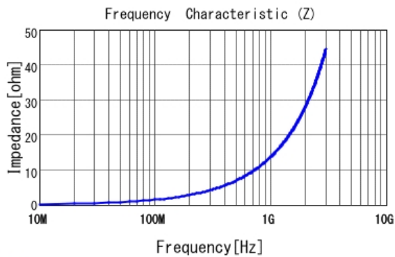
■ LQP03TG2N2C02 |Z|
