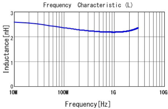
■ LQP03TG2N2C02 L
