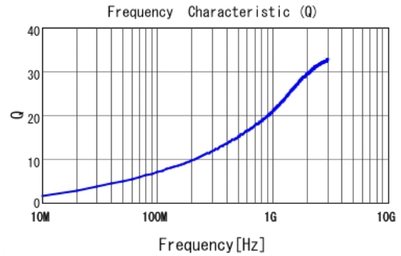
■ LQP03TG2N2C02 Q
