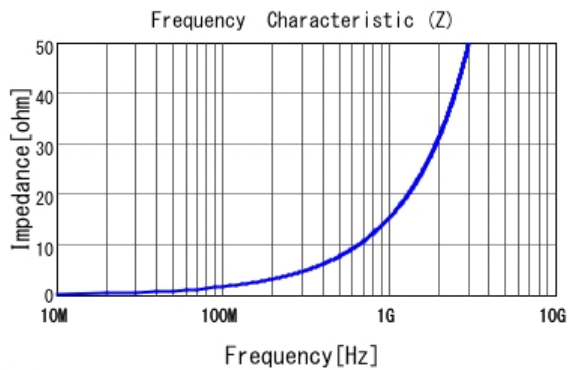
■ LQP03TG2N4B02 |Z|
