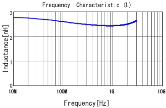
■ LQP03TG2N4C02 L
