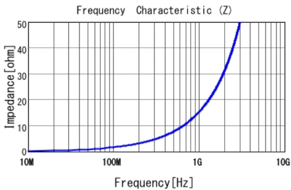
■ LQP03TG2N4C02 |Z|
