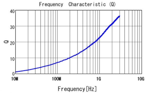
■ LQP03TG2N4C02 Q
