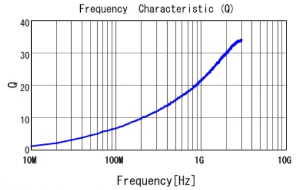
■ LQP03TG2N5B02 Q
