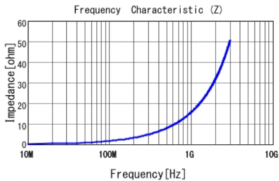
■ LQP03TG2N5B02 |Z|
