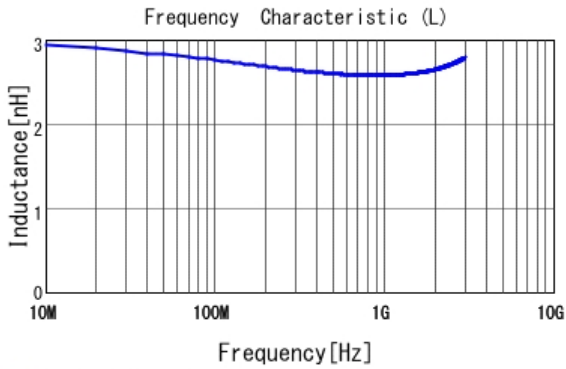
■ LQP03TG2N6B02 L
