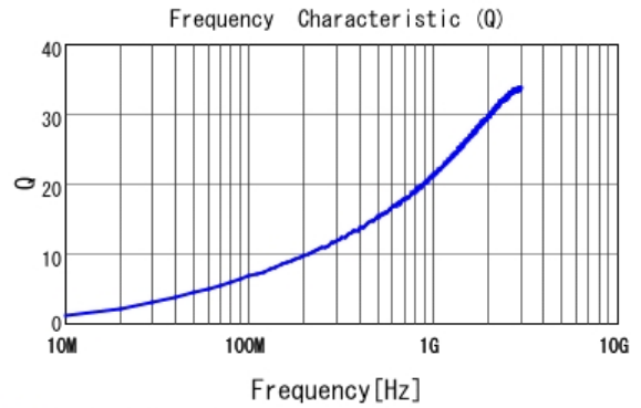
■ LQP03TG2N6B02 Q
