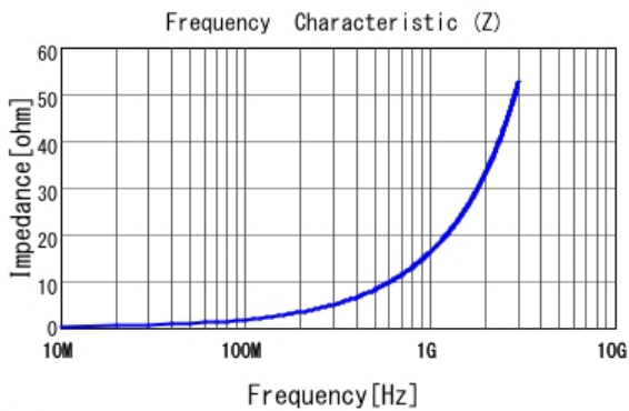
■ LQP03TG2N6B02 |Z|
