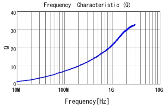
■ LQP03TG2N7B02 Q
