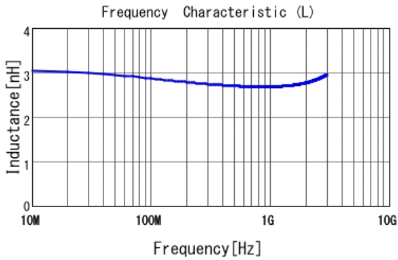
■ LQP03TG2N7B02 L
