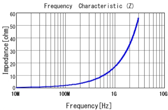
■ LQP03TG2N7B02 |Z|
