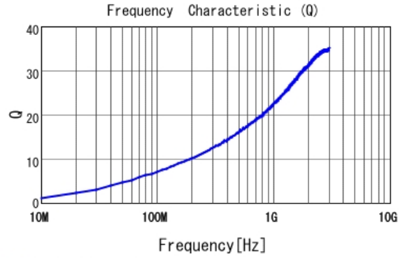
■ LQP03TG2N9B02 Q
