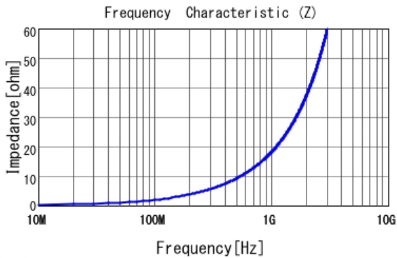
■ LQP03TG2N9B02 |Z|
