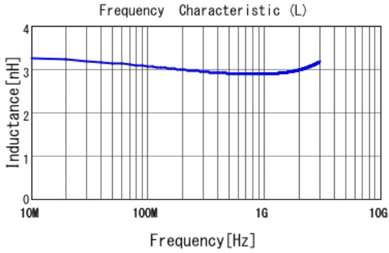
■ LQP03TG2N9B02 L
