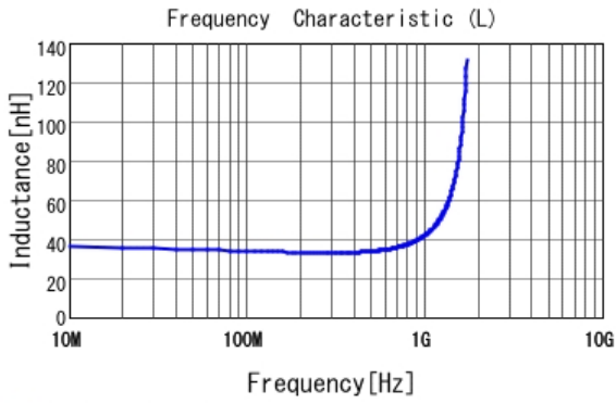
■ LQP03TG33NJ02 L
