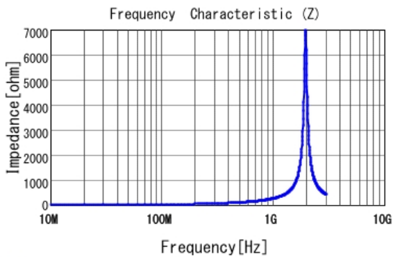
■ LQP03TG33NJ02 |Z|
