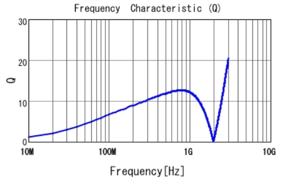
■ LQP03TG33NJ02 Q
