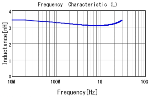
■ LQP03TG3N1B02 L
