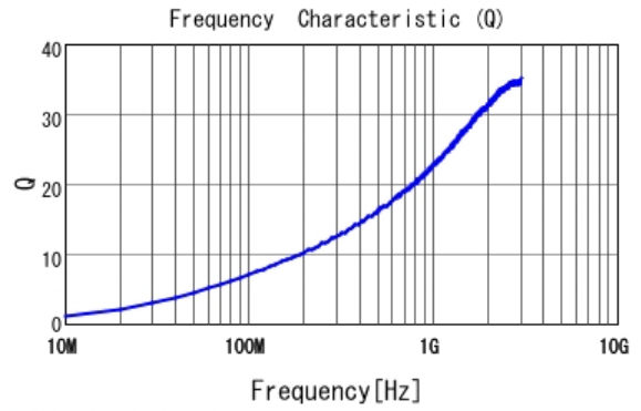
■ LQP03TG3N1B02 Q
