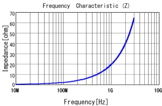
■ LQP03TG3N1B02 |Z|
