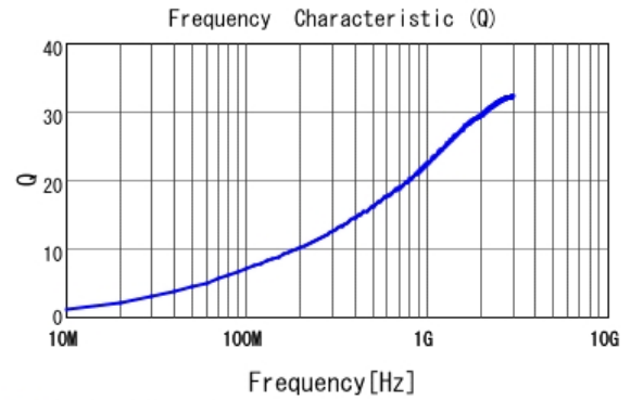
■ LQP03TG3N6B02 Q
