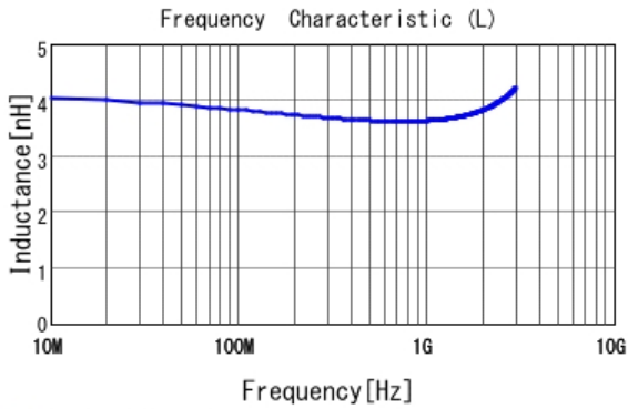
■ LQP03TG3N6B02 L
