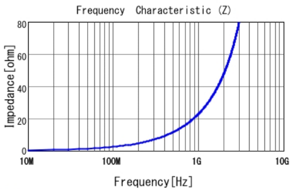
■ LQP03TG3N6C02 |Z|
