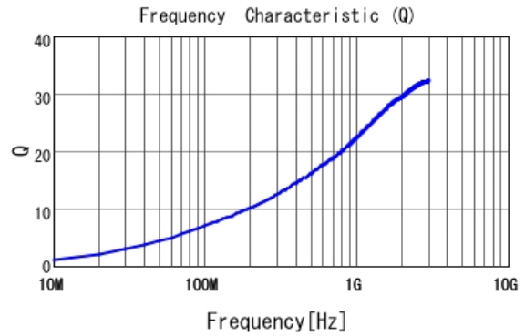
■ LQP03TG3N6C02 Q
