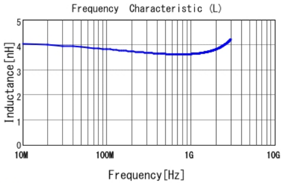
■ LQP03TG3N6C02 L
