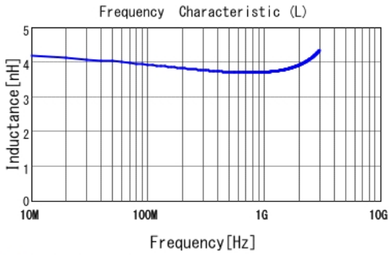
■ LQP03TG3N7B02 L
