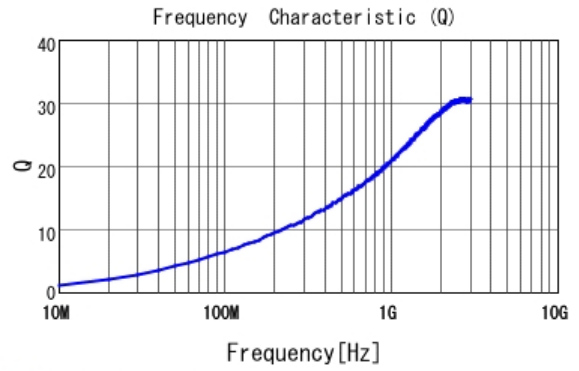
■ LQP03TG3N7B02 Q
