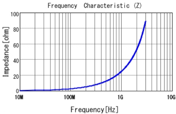
■ LQP03TG3N9B02 |Z|
