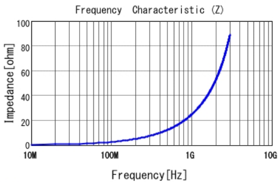
■ LQP03TG3N9C02 |Z|
