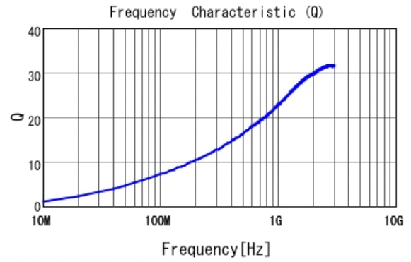
■ LQP03TG3N9C02 Q
