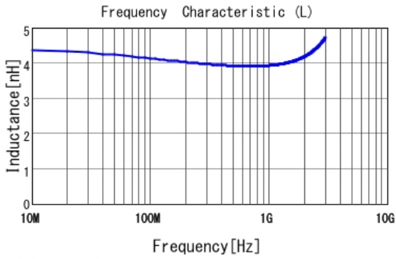
■ LQP03TG3N9C02 L
