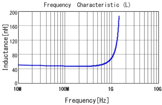
■ LQP03TG47NJ02 L
