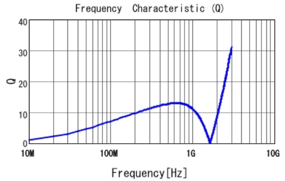
■ LQP03TG47NJ02 Q
