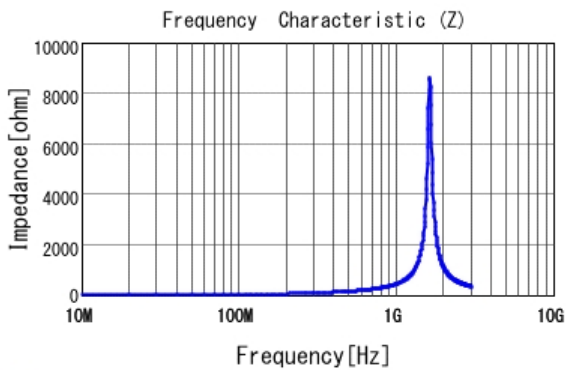
■ LQP03TG47NJ02 |Z|
