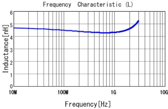
■ LQP03TG4N3J02 L
