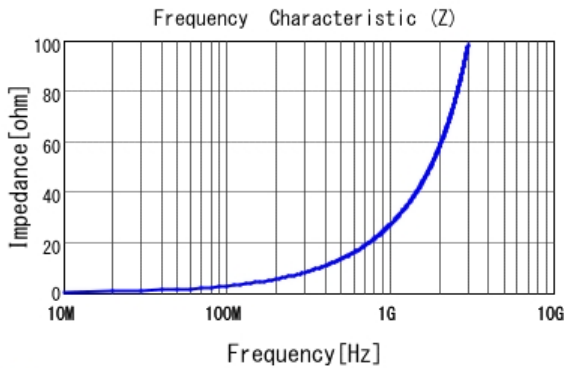
■ LQP03TG4N3J02 |Z|
