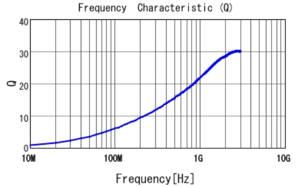
■ LQP03TG4N3J02 Q
