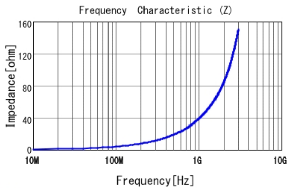
■ LQP03TG6N2J02 |Z|
