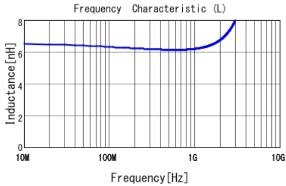
■ LQP03TG6N2J02 L
