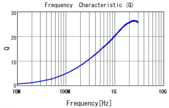
■ LQP03TG6N2J02 Q
