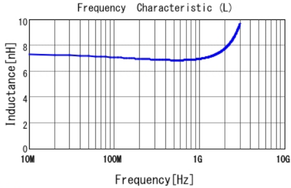
■ LQP03TG6N8J02 L
