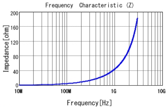
■ LQP03TG6N8J02 |Z|
