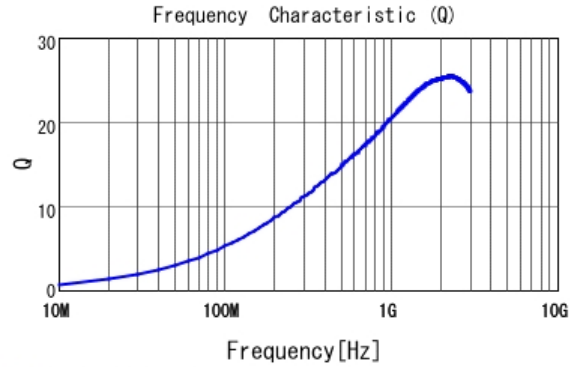
■ LQP03TG6N8J02 Q
