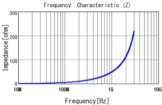
■ LQP03TG7N5J02 |Z|
