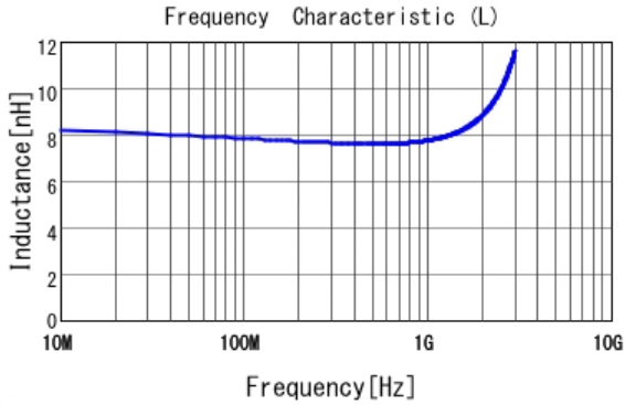
■ LQP03TG7N5J02 L
