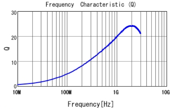
■ LQP03TG7N5J02 Q
