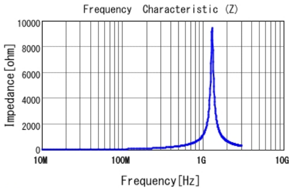
■ LQP03TG82NJ02 |Z|
