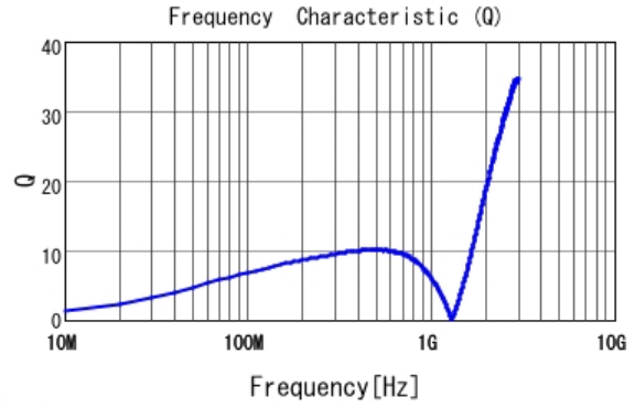
■ LQP03TG82NJ02 Q
