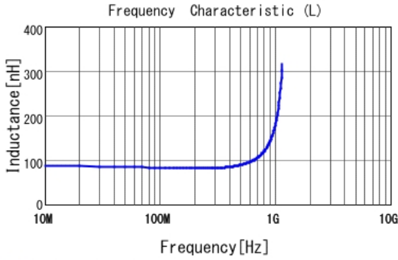
■ LQP03TG82NJ02 L
