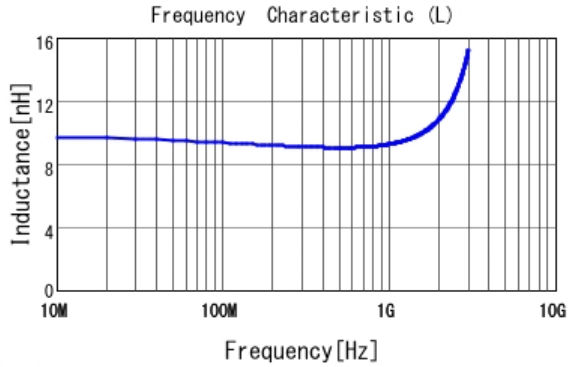
■ LQP03TG9N1H02 L
