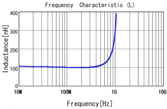
■ LQP03TGR10J02 L
