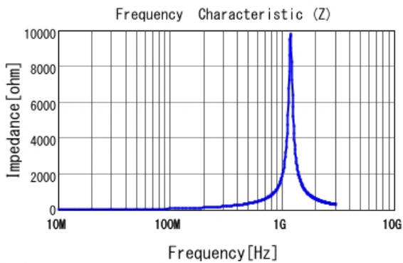
■ LQP03TGR10J02 |Z|
