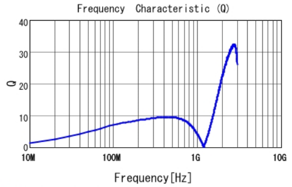
■ LQP03TGR10J02 Q
