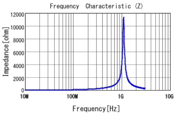
■ LQP03TGR12J02 |Z|
