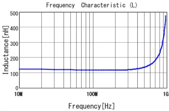
■ LQP03TGR12J02 L
