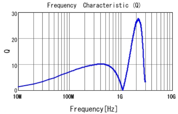
■ LQP03TGR12J02 Q
