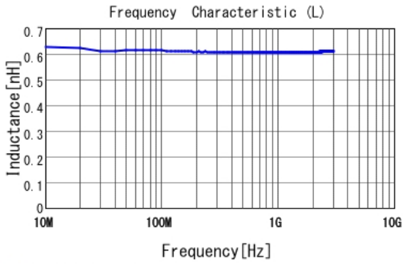
■ LQP03TN0N6C02 L
