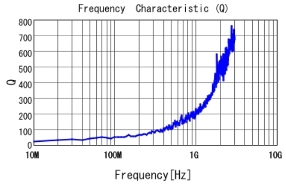
■ LQP03TN0N6C02 Q
