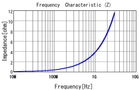
■ LQP03TN0N6C02 |Z|
