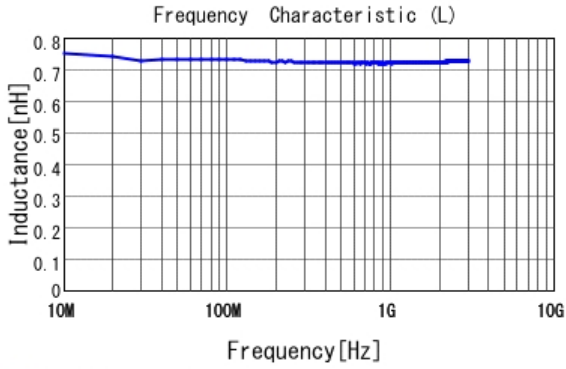
■ LQP03TN0N7B02 L
