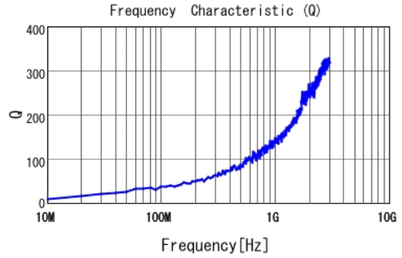
■ LQP03TN0N7B02 Q
