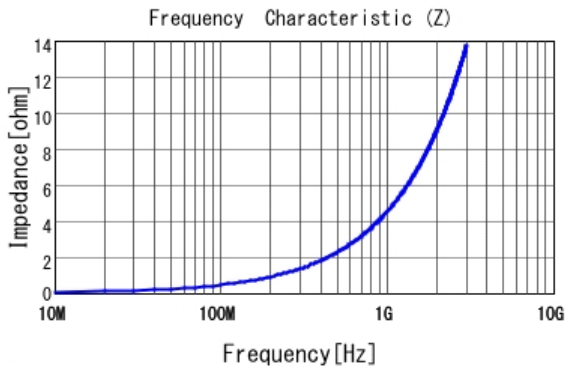
■ LQP03TN0N7B02 |Z|
